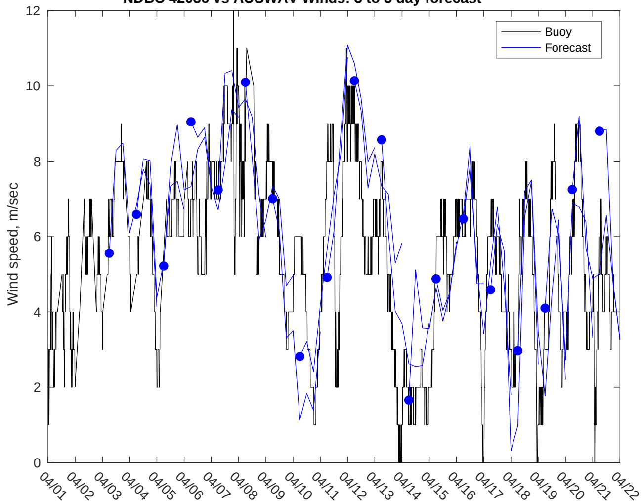
NDBC 42036 vs AUSWAV Winds: 3 to 5 day forecast
