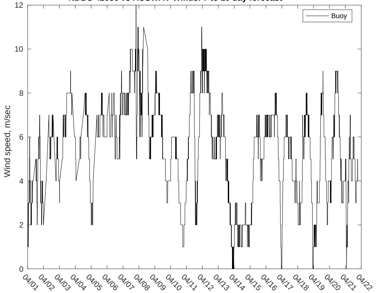
NDBC 42036 vs AUSWAV Winds: 7 to 10 day forecast
