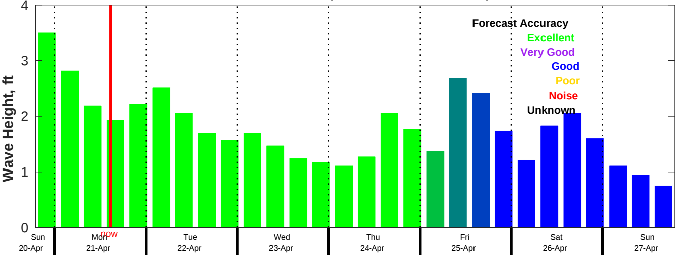
AUSWAV Wave Forecast for NDBC 42036 from 20-Apr-2025 19:00:00 to 27-Apr-2025 19:00:00
