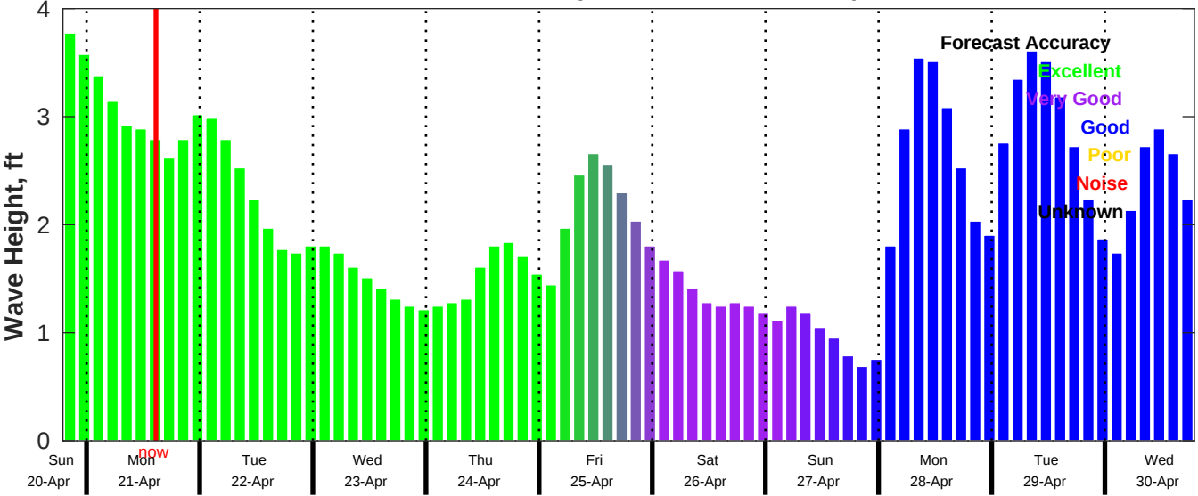
CMEMS Wave Forecast for NDBC 42036 from 20-Apr-2025 19:00:00 to 30-Apr-2025 19:00:00
