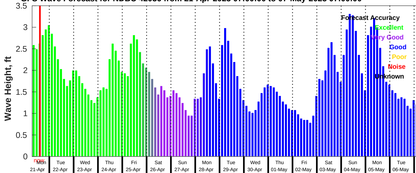
GFS Wave Forecast for NDBC 42036 from 21-Apr-2025 07:00:00 to 07-May-2025 07:00:00
