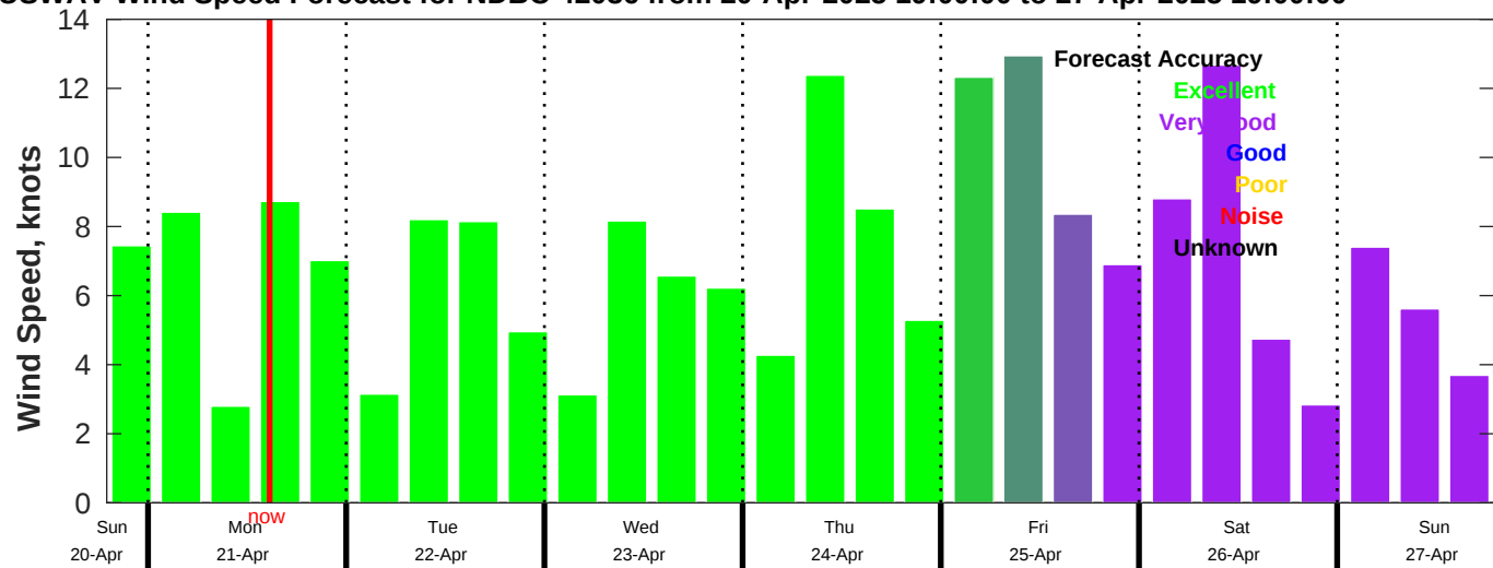
AUSWAV Wind Speed Forecast for NDBC 42036 from 20-Apr-2025 19:00:00 to 27-Apr-2025 19:00:00
