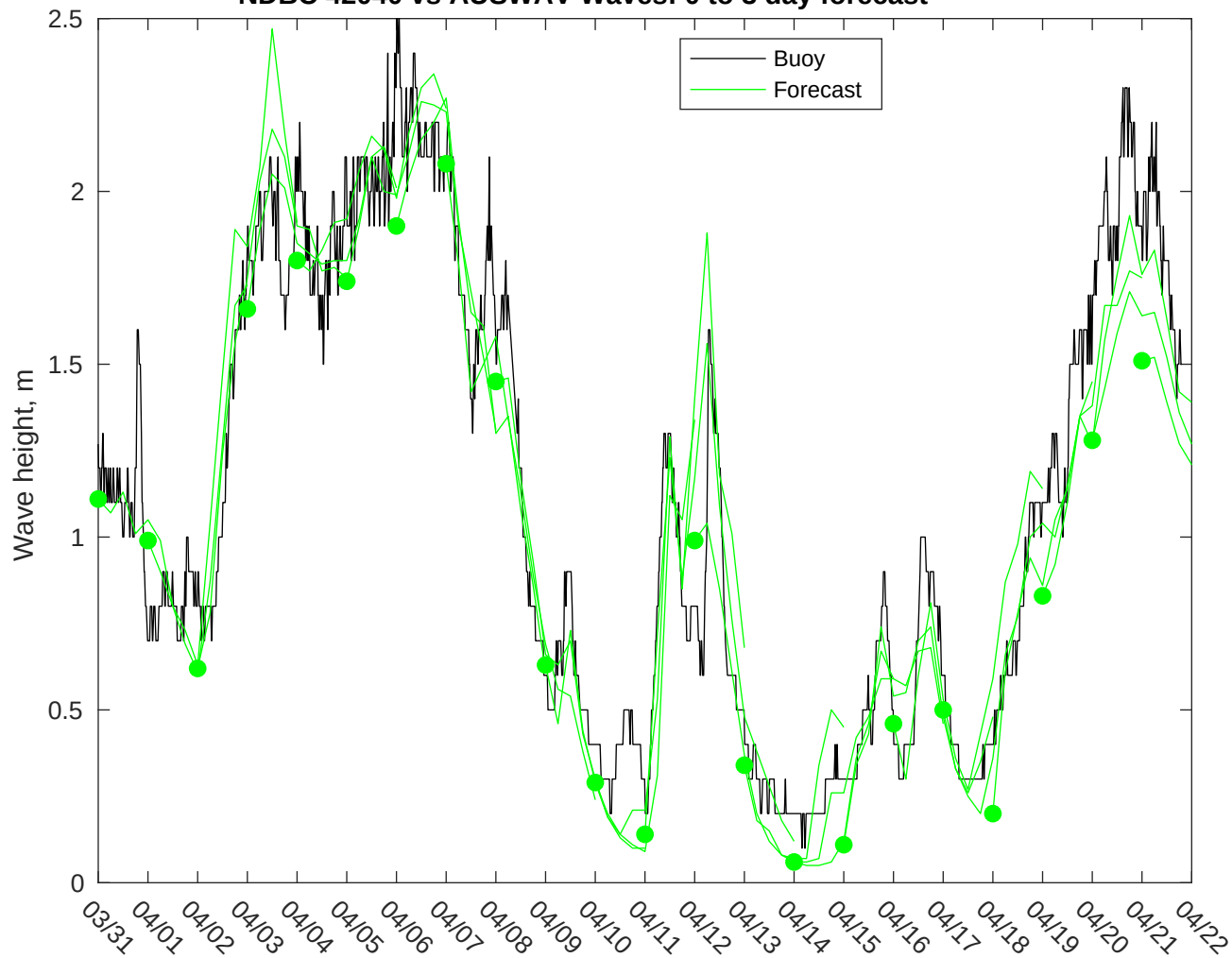
NDBC 42040 vs AUSWAV Waves: 0 to 3 day forecast
