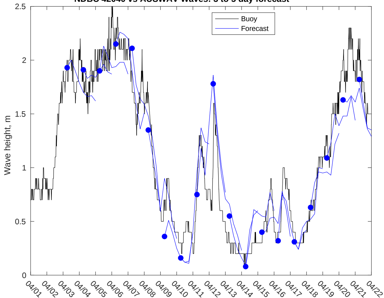
NDBC 42040 vs AUSWAV Waves: 3 to 5 day forecast
