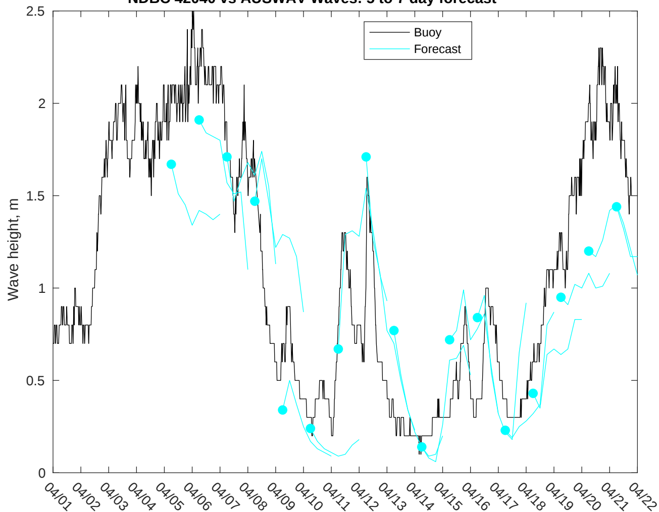
NDBC 42040 vs AUSWAV Waves: 5 to 7 day forecast
