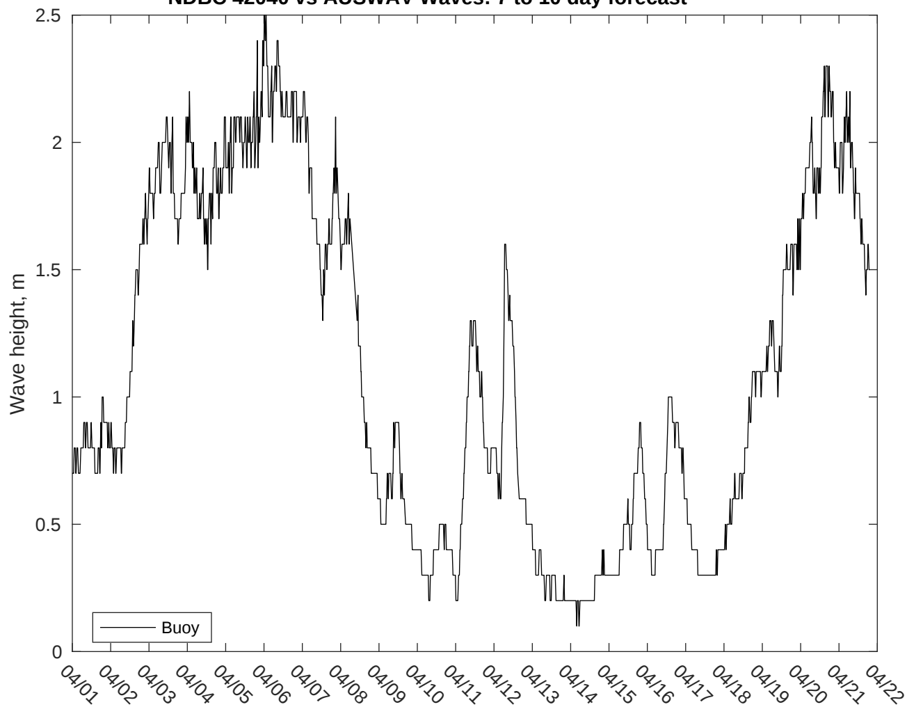
NDBC 42040 vs AUSWAV Waves: 7 to 10 day forecast
