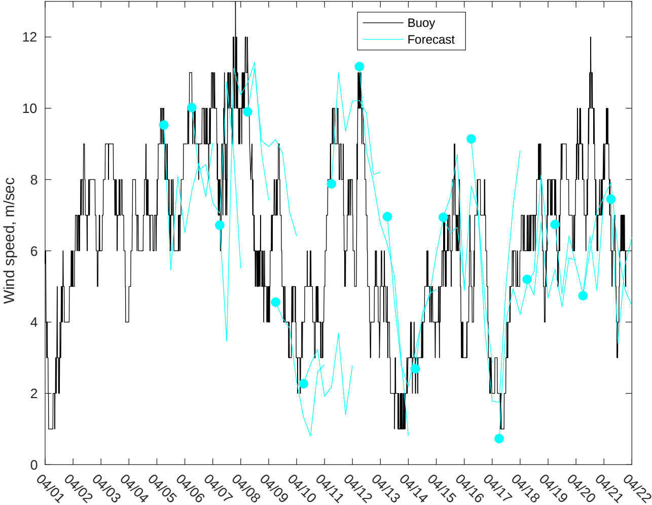
NDBC 42040 vs AUSWAV Winds: 5 to 7 day forecast
