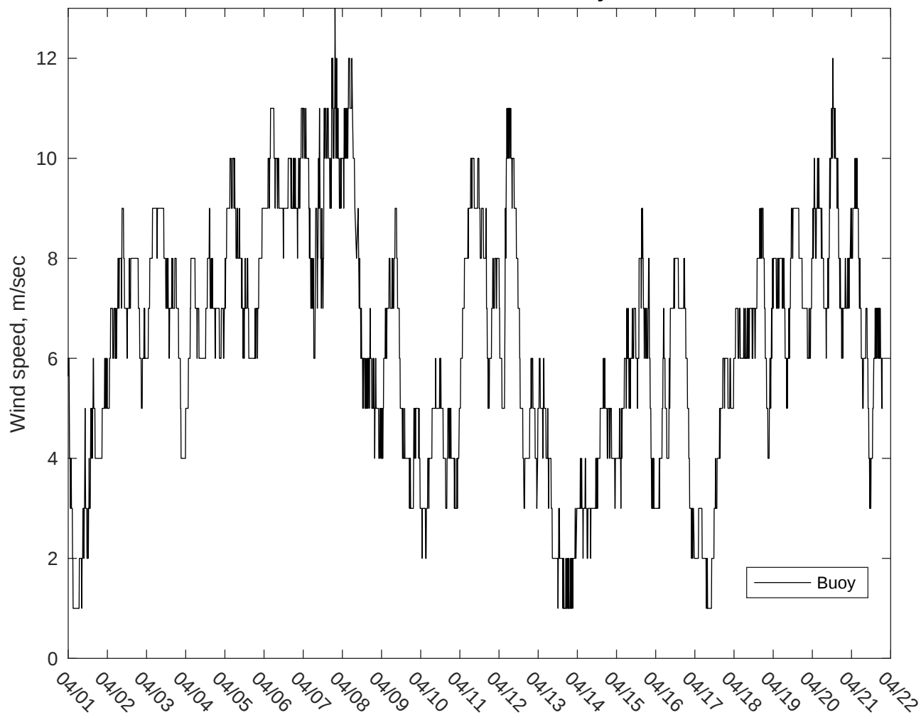
NDBC 42040 vs AUSWAV Winds: 7 to 10 day forecast
