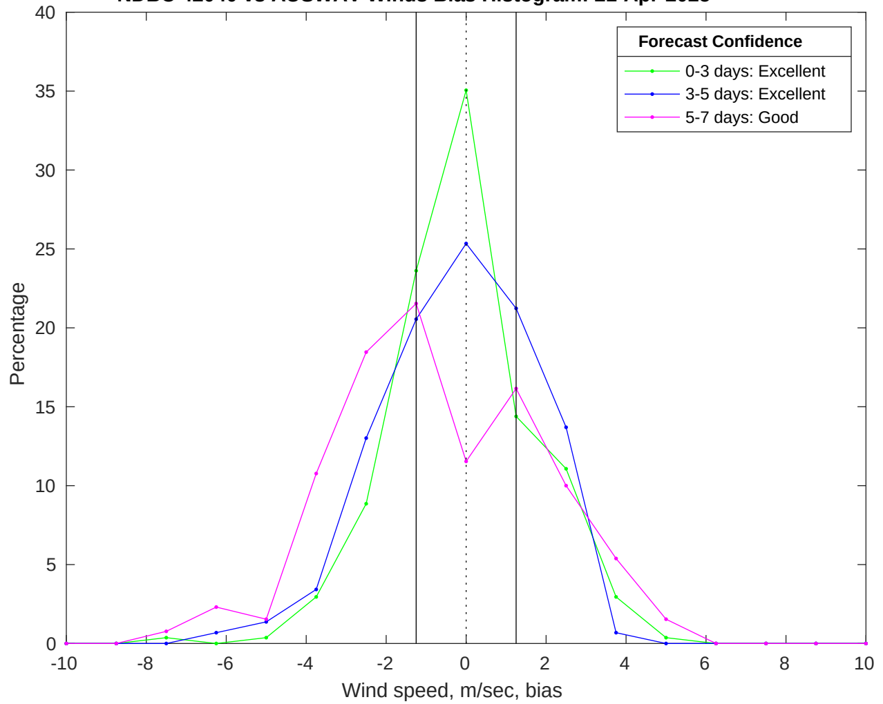
NDBC 42040 vs AUSWAV Winds Bias Histogram: 21-Apr-2025
