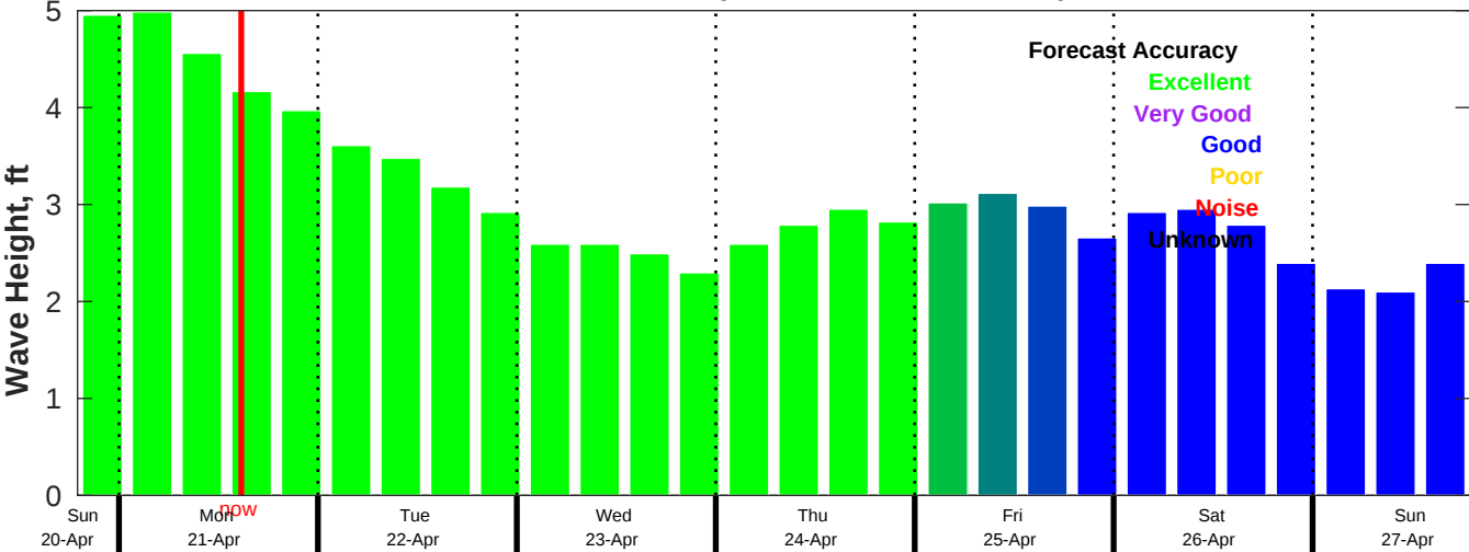
AUSWAV Wave Forecast for NDBC 42040 from 20-Apr-2025 19:00:00 to 27-Apr-2025 19:00:00
