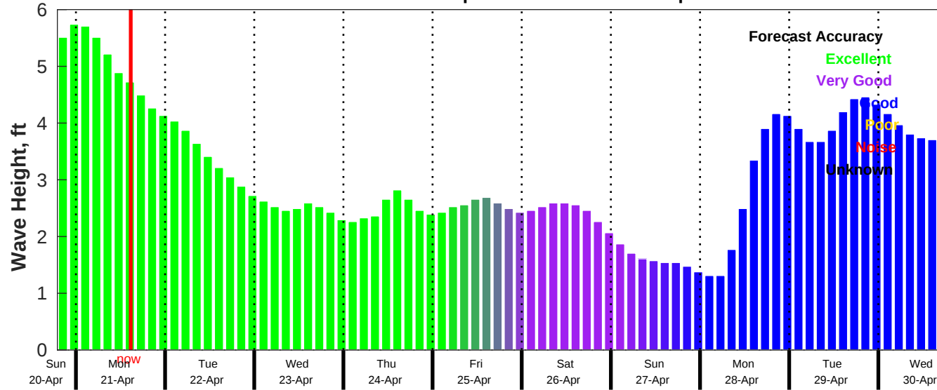
CMEMS Wave Forecast for NDBC 42040 from 20-Apr-2025 19:00:00 to 30-Apr-2025 19:00:00
