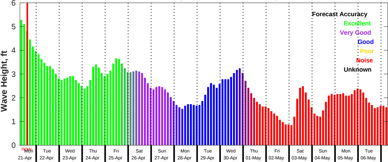
GFS Wave Forecast for NDBC 42040 from 21-Apr-2025 07:00:00 to 07-May-2025 07:00:00
