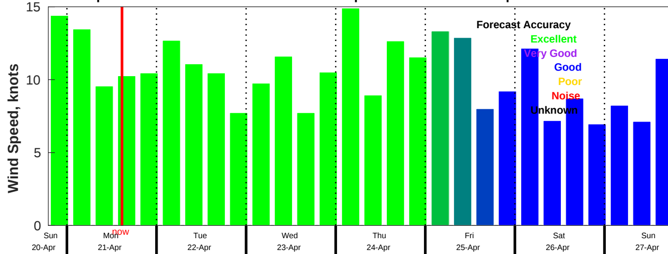
AUSWAV Wind Speed Forecast for NDBC 42040 from 20-Apr-2025 19:00:00 to 27-Apr-2025 19:00:00
