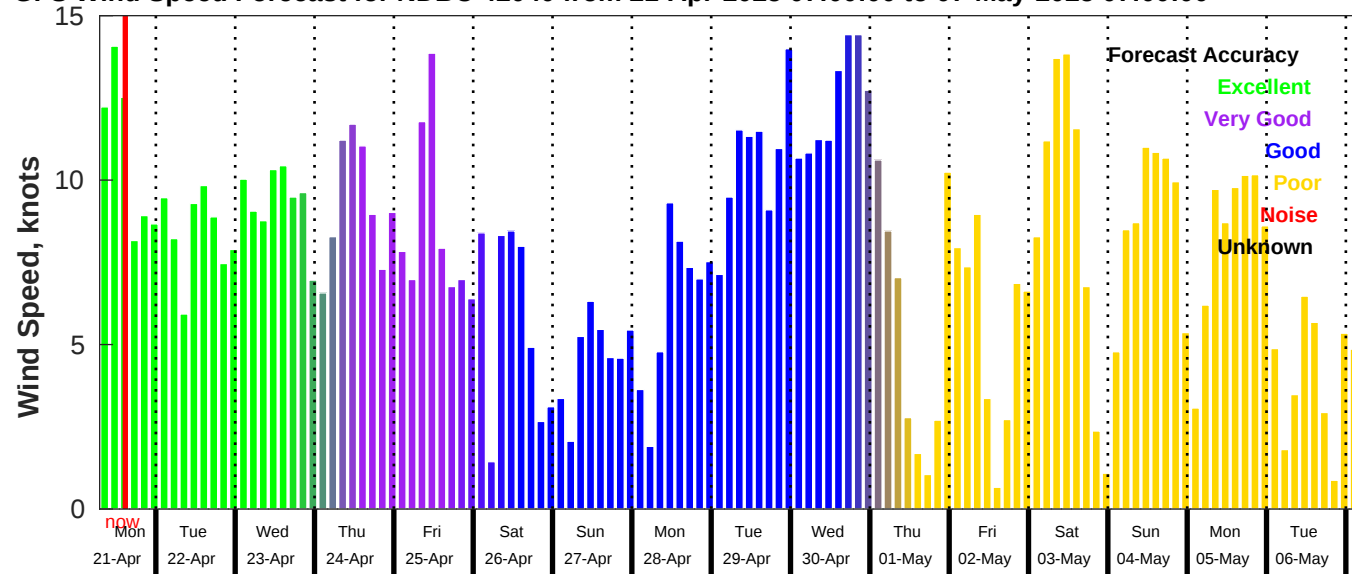
GFS Wind Speed Forecast for NDBC 42040 from 21-Apr-2025 07:00:00 to 07-May-2025 07:00:00
