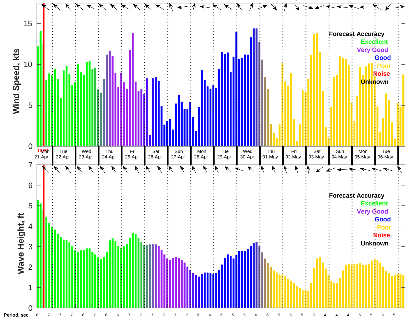
Wind & Wave Forecast for NDBC 42040 from 21-Apr-2025 07:00:00 to 07-May-2025 07:00:00
