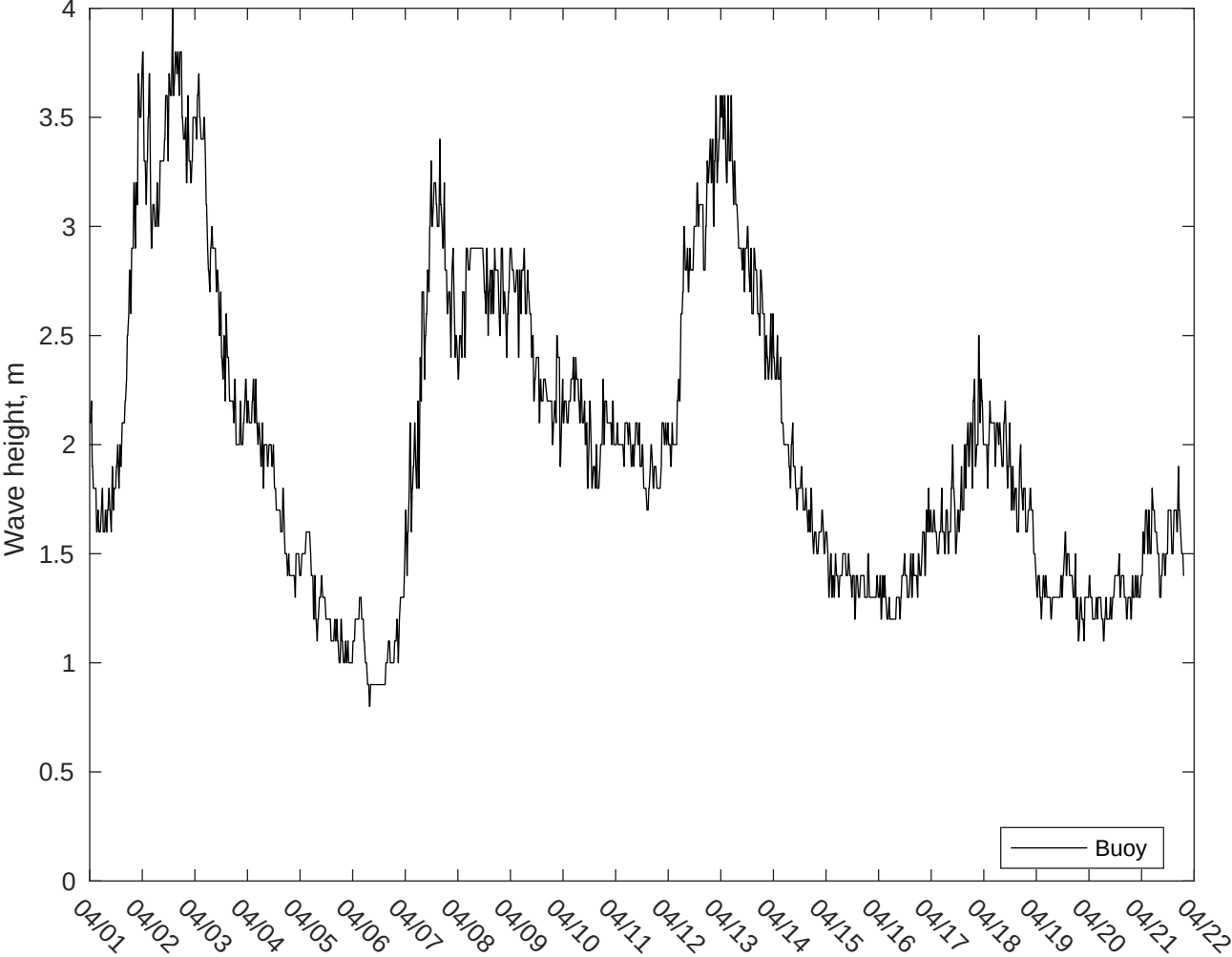
NDBC 46011 vs AUSWAV Waves: 7 to 10 day forecast
