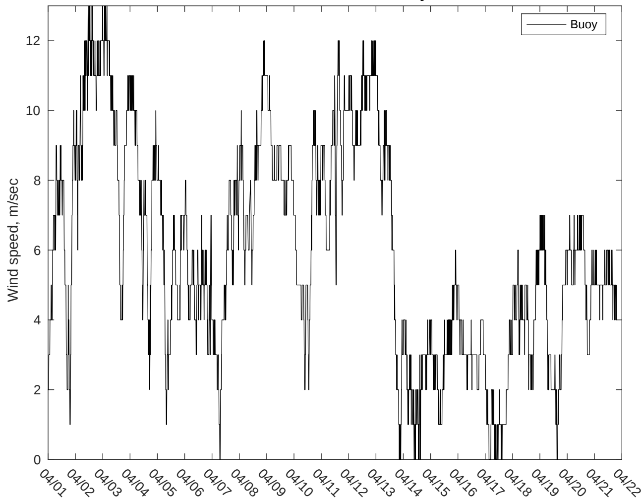
NDBC 46011 vs AUSWAV Winds: 10 to 16 day forecast
