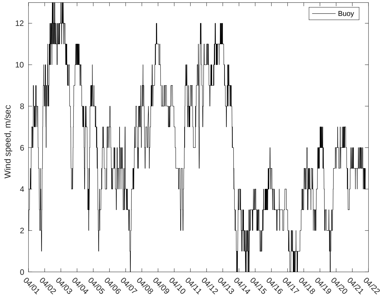
NDBC 46011 vs AUSWAV Winds: 7 to 10 day forecast
