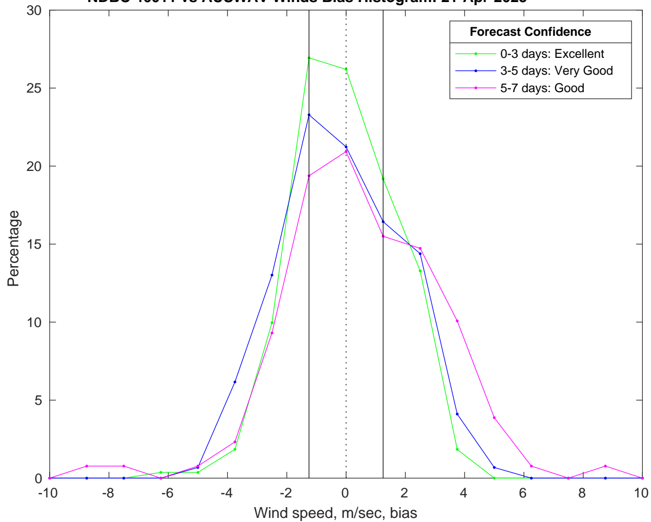
NDBC 46011 vs AUSWAV Winds Bias Histogram: 21-Apr-2025
