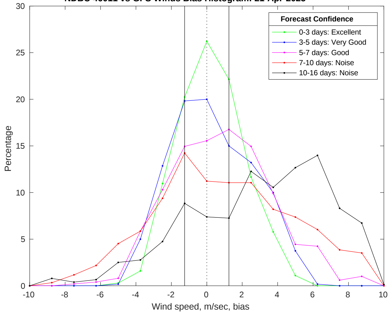
NDBC 46011 vs GFS Winds Bias Histogram: 21-Apr-2025
