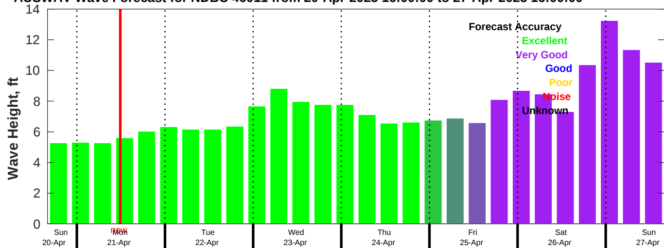
AUSWAV Wave Forecast for NDBC 46011 from 20-Apr-2025 16:00:00 to 27-Apr-2025 16:00:00
