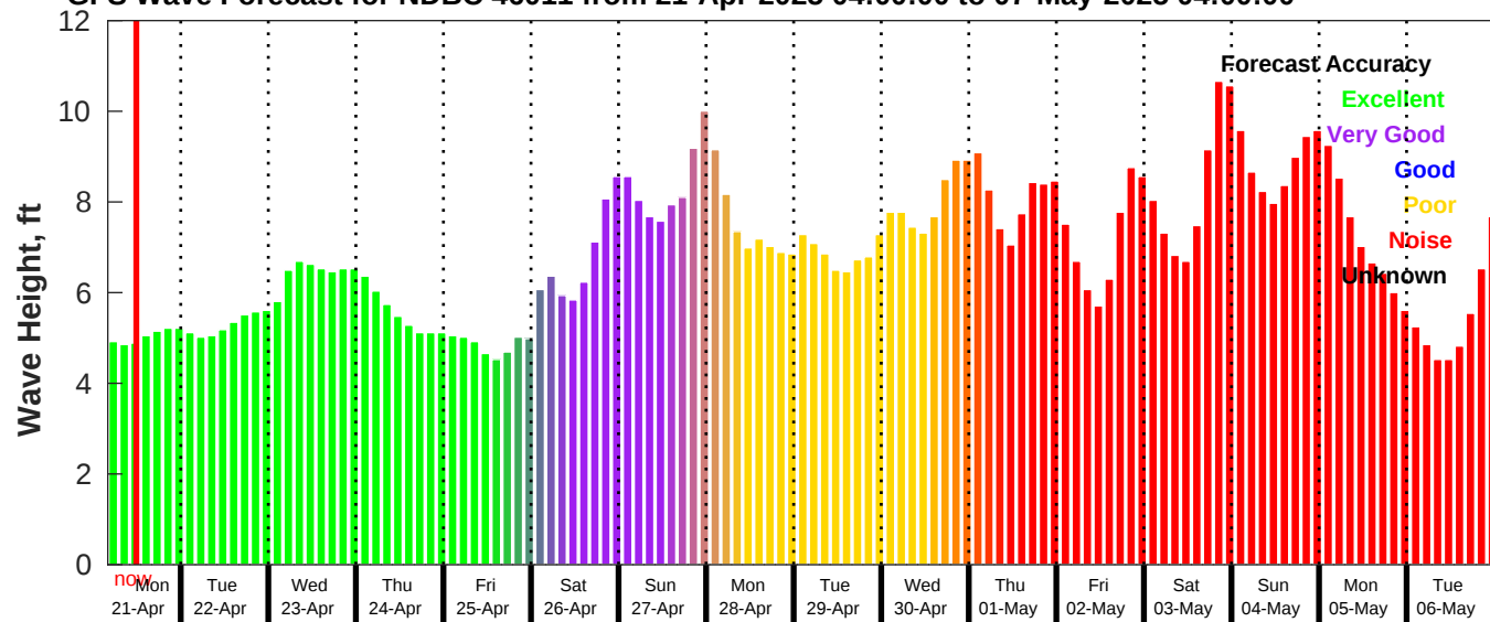
GFS Wave Forecast for NDBC 46011 from 21-Apr-2025 04:00:00 to 07-May-2025 04:00:00
