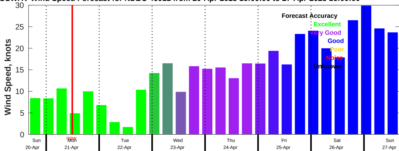
AUSWAV Wind Speed Forecast for NDBC 46011 from 20-Apr-2025 16:00:00 to 27-Apr-2025 16:00:00
