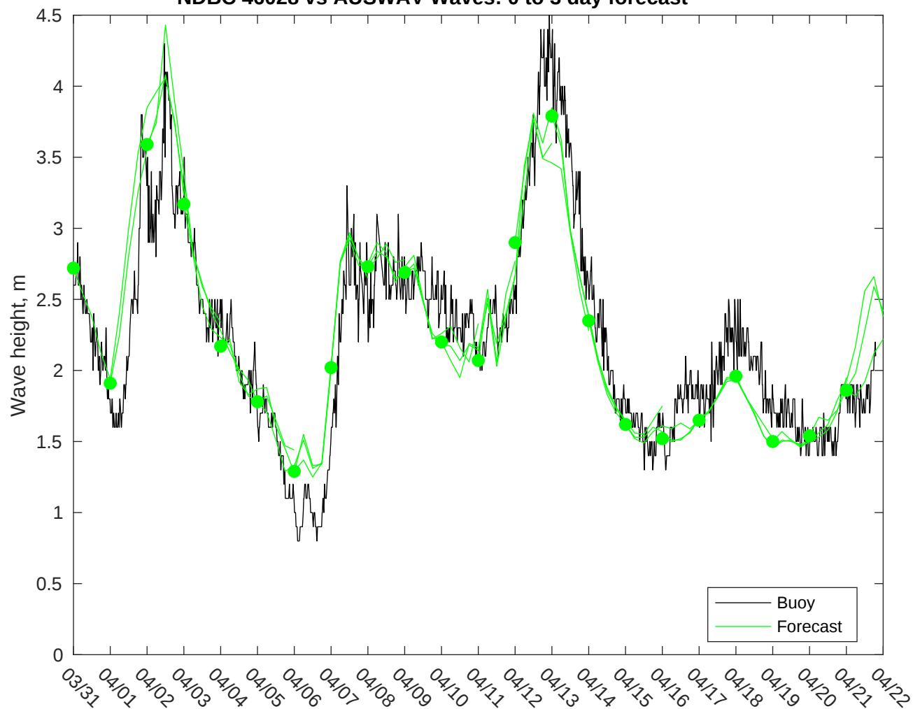
NDBC 46028 vs AUSWAV Waves: 0 to 3 day forecast
