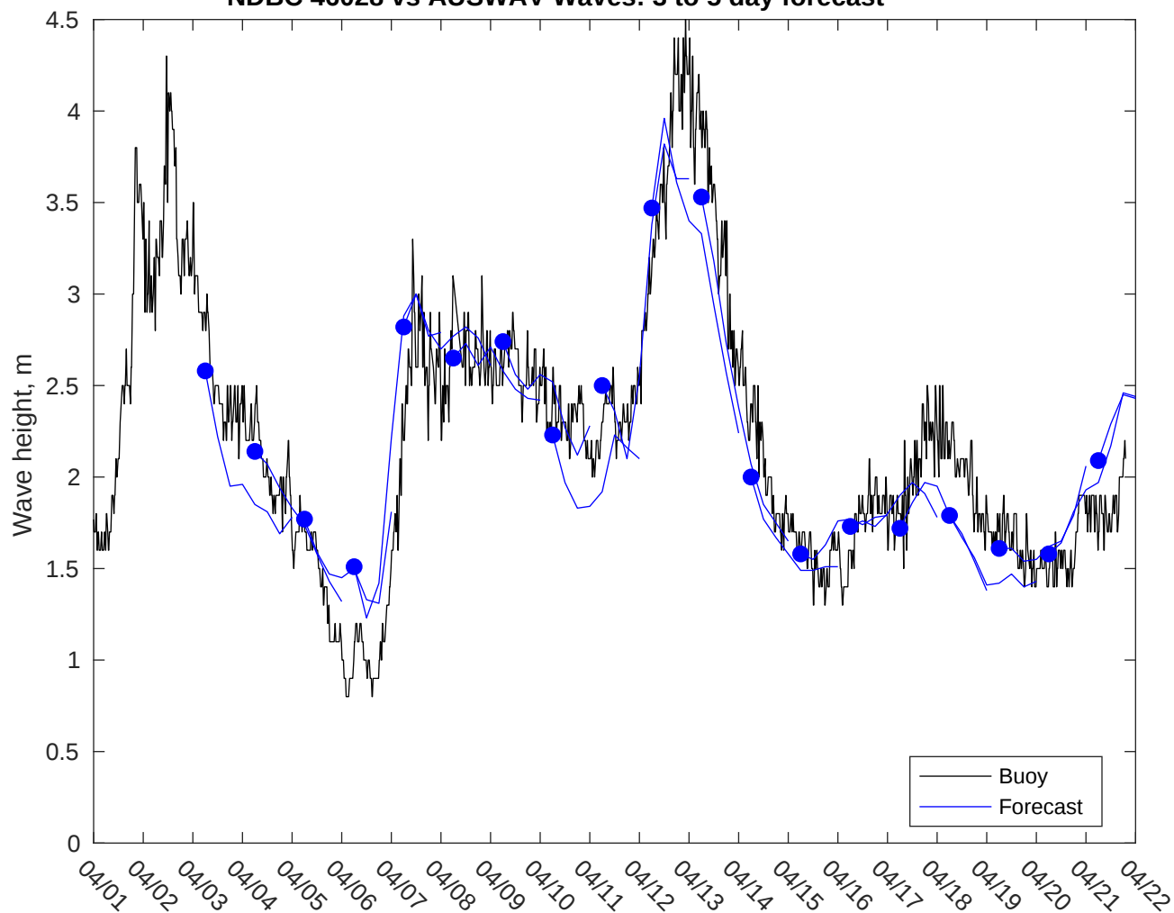
NDBC 46028 vs AUSWAV Waves: 3 to 5 day forecast
