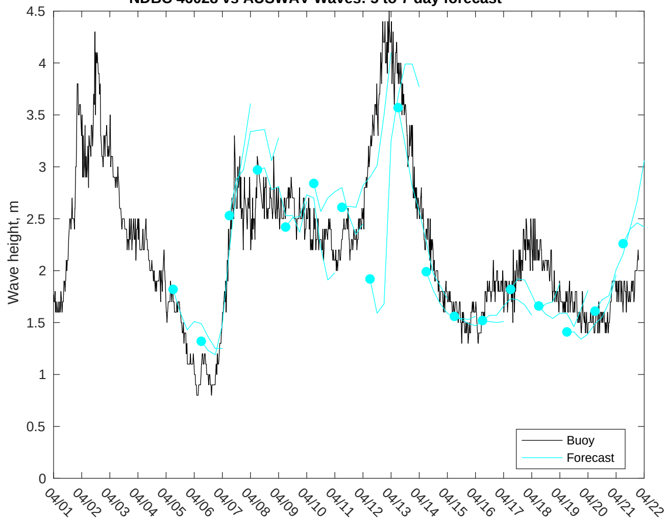
NDBC 46028 vs AUSWAV Waves: 5 to 7 day forecast
