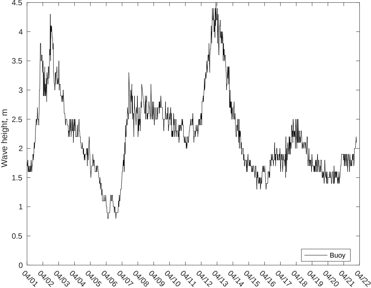
NDBC 46028 vs AUSWAV Waves: 7 to 10 day forecast
