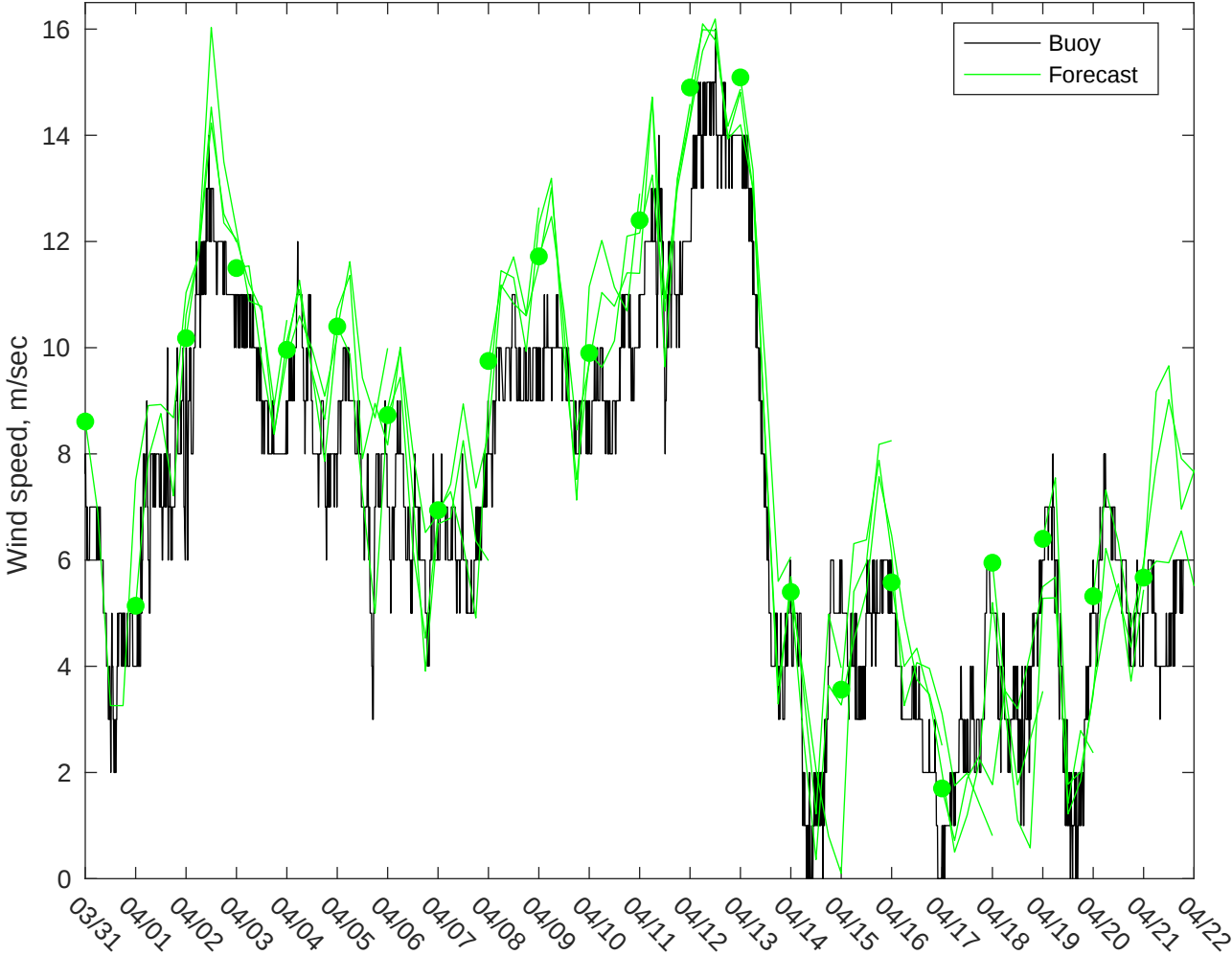
NDBC 46028 vs AUSWAV Winds: 0 to 3 day forecast
