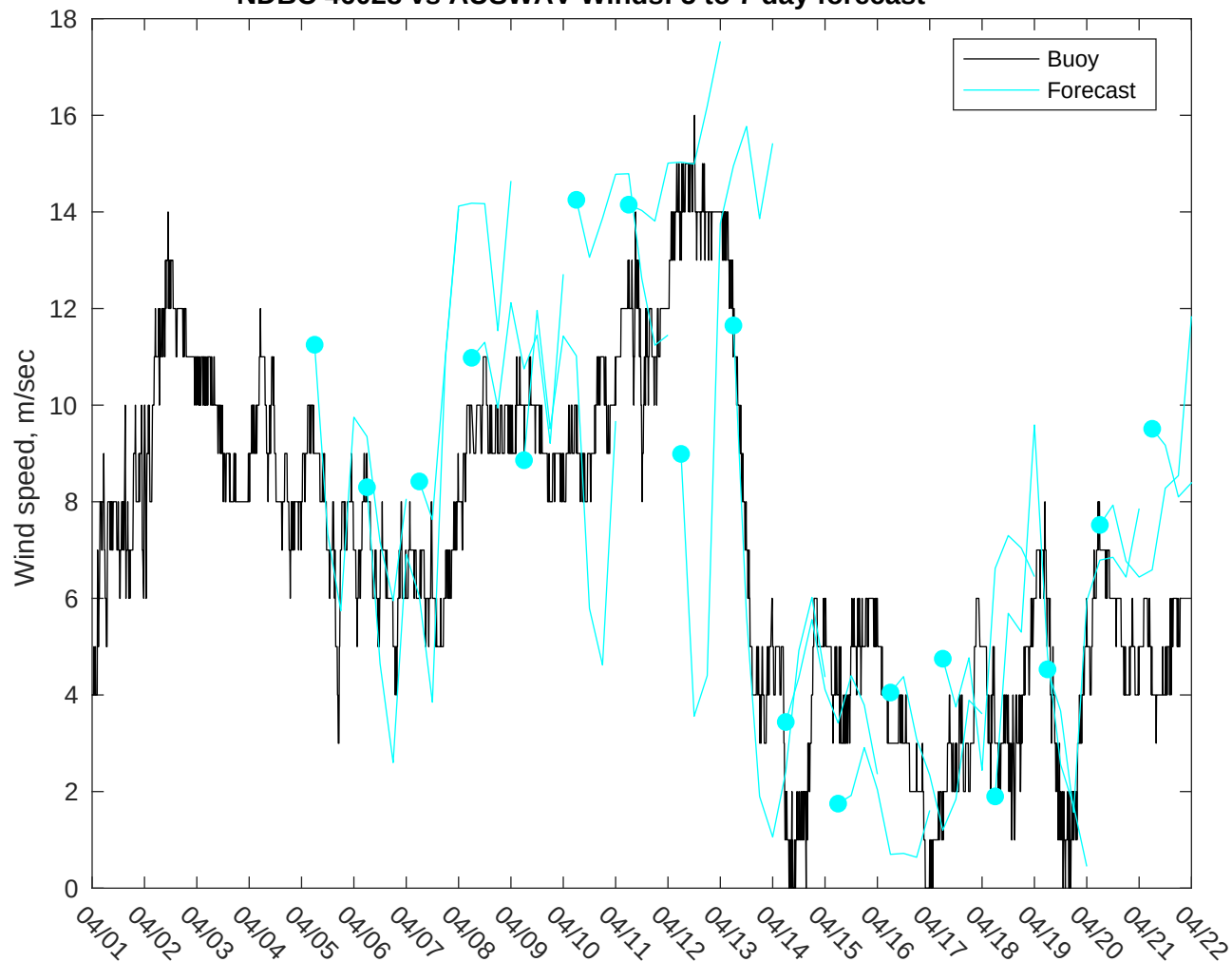
NDBC 46028 vs AUSWAV Winds: 5 to 7 day forecast
