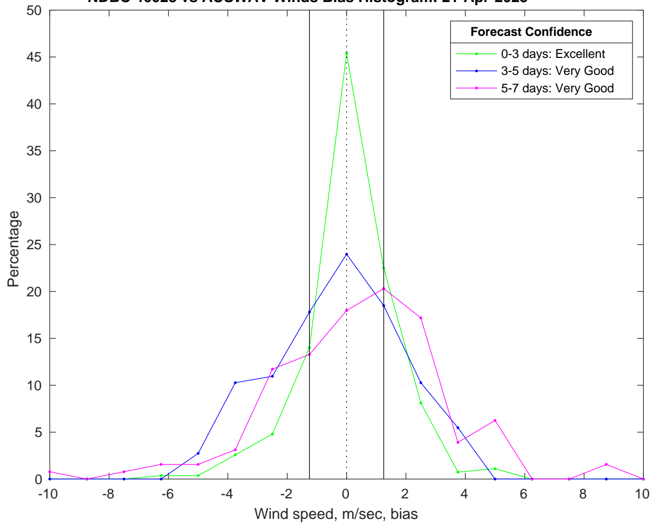
NDBC 46028 vs AUSWAV Winds Bias Histogram: 21-Apr-2025
