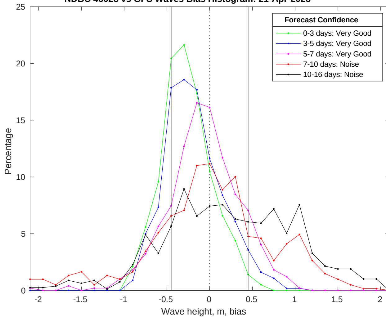
NDBC 46028 vs GFS Waves Bias Histogram: 21-Apr-2025
