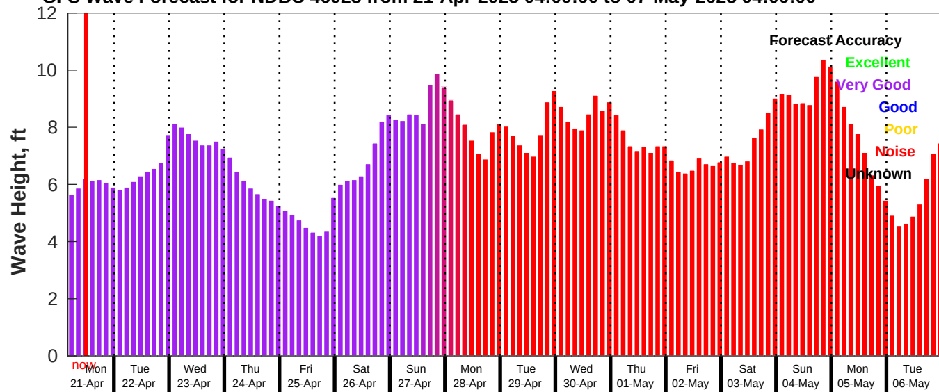
GFS Wave Forecast for NDBC 46028 from 21-Apr-2025 04:00:00 to 07-May-2025 04:00:00
