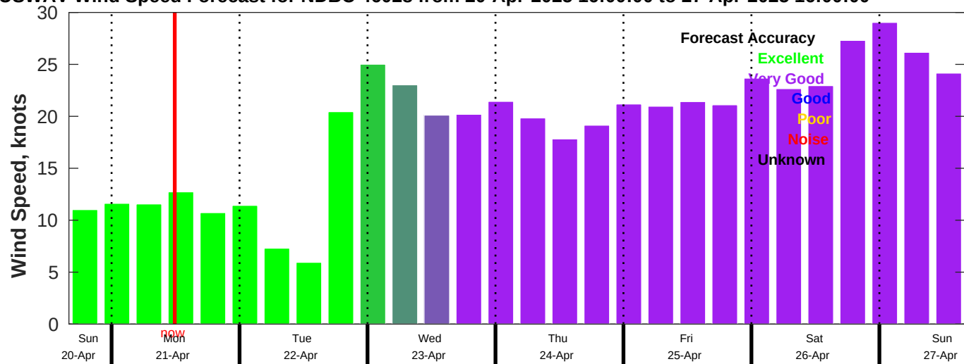
AUSWAV Wind Speed Forecast for NDBC 46028 from 20-Apr-2025 16:00:00 to 27-Apr-2025 16:00:00
