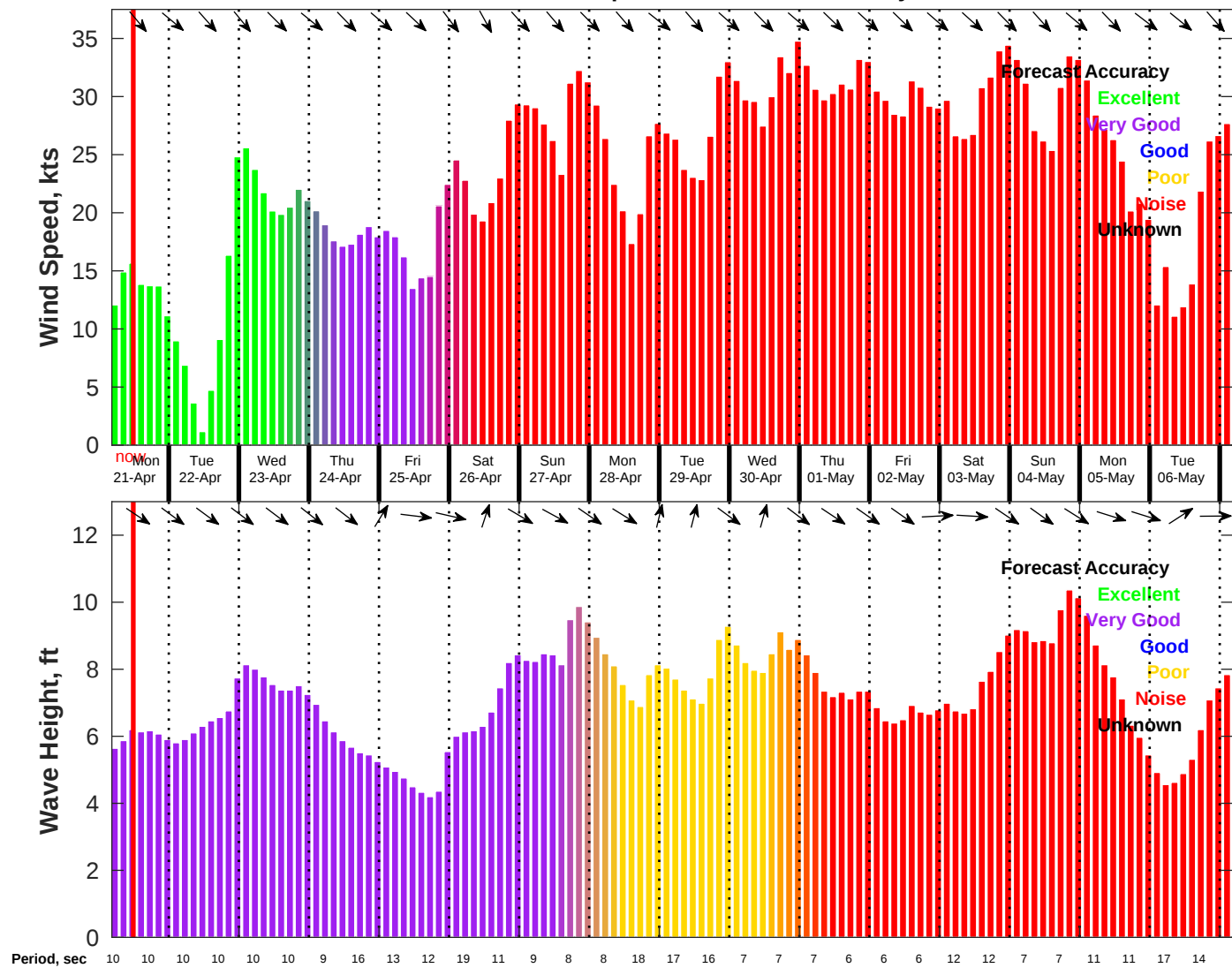
Wind & Wave Forecast for NDBC 46028 from 21-Apr-2025 04:00:00 to 07-May-2025 04:00:00
