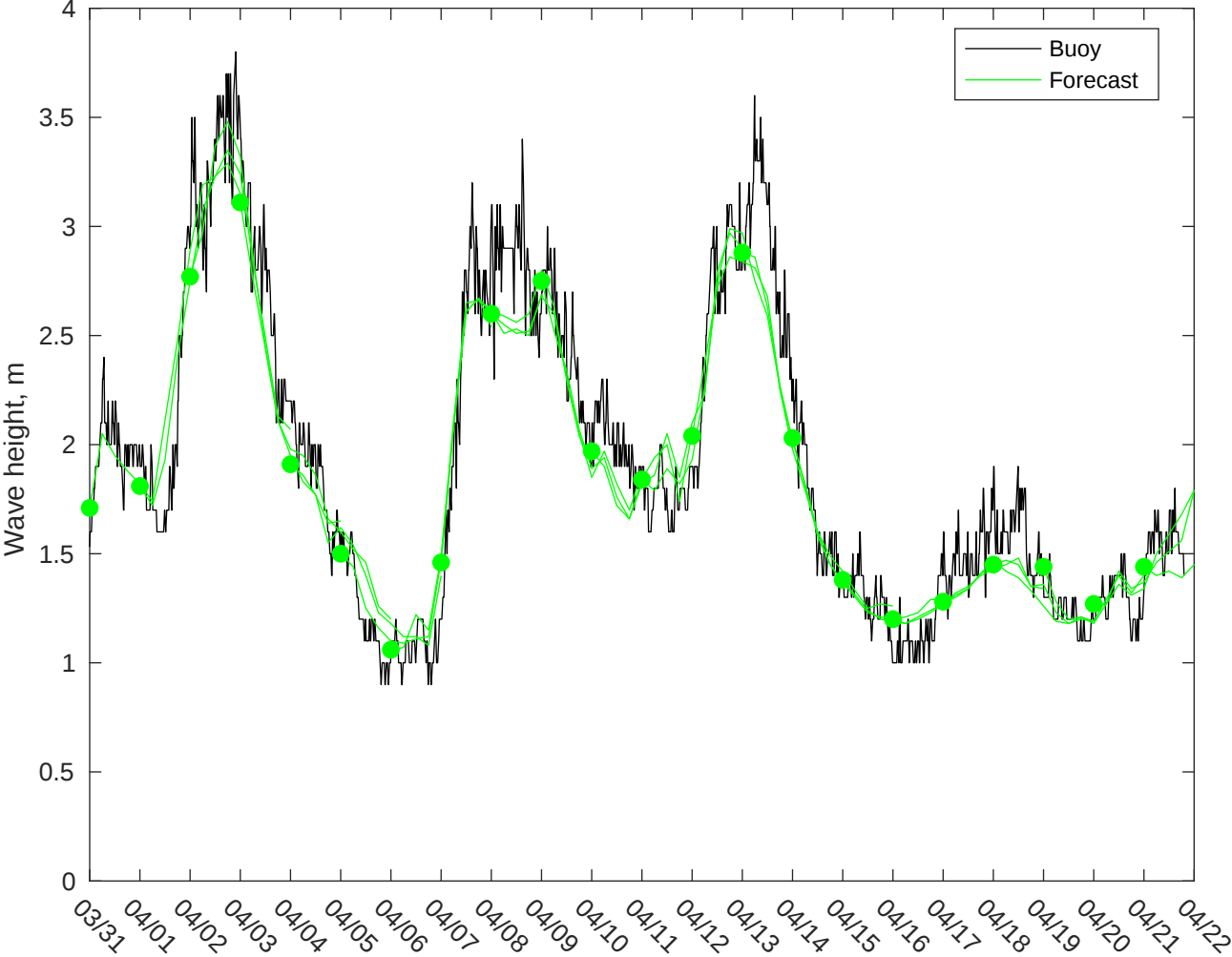
NDBC 46054 vs AUSWAV Waves: 0 to 3 day forecast
