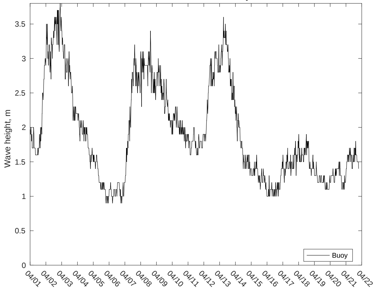
NDBC 46054 vs AUSWAV Waves: 10 to 16 day forecast
