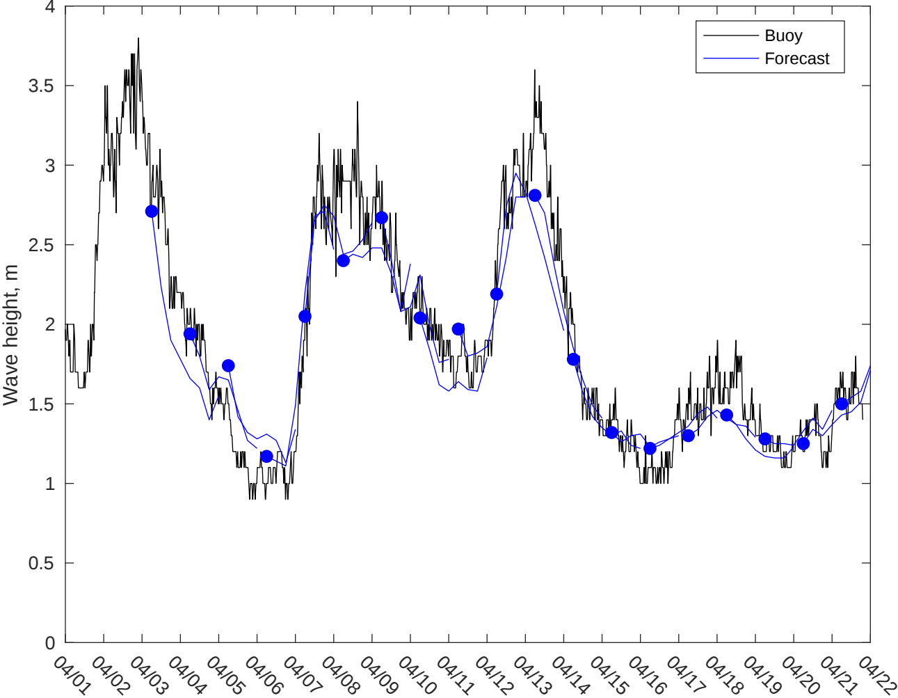
NDBC 46054 vs AUSWAV Waves: 3 to 5 day forecast
