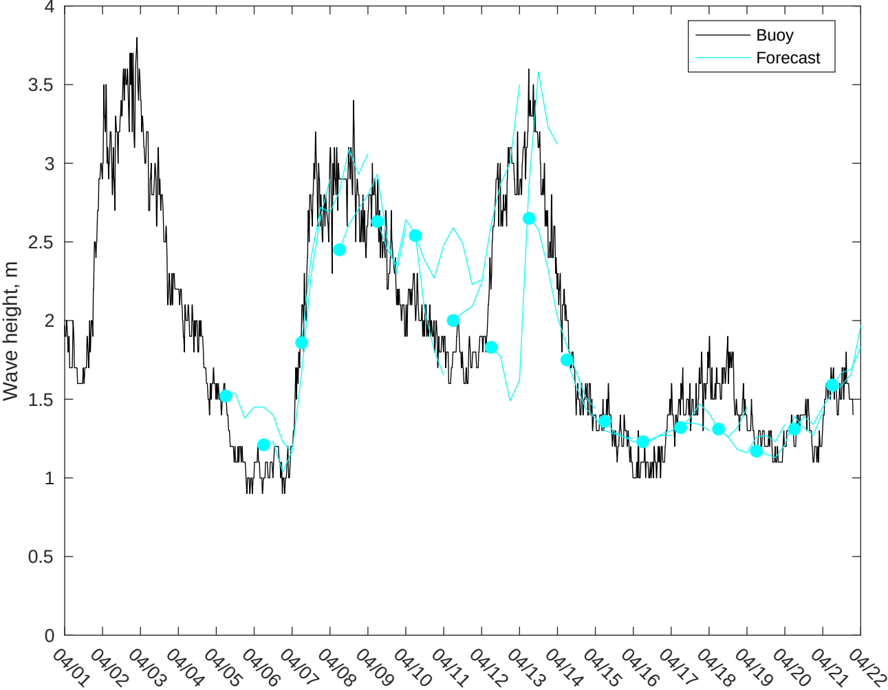
NDBC 46054 vs AUSWAV Waves: 5 to 7 day forecast
