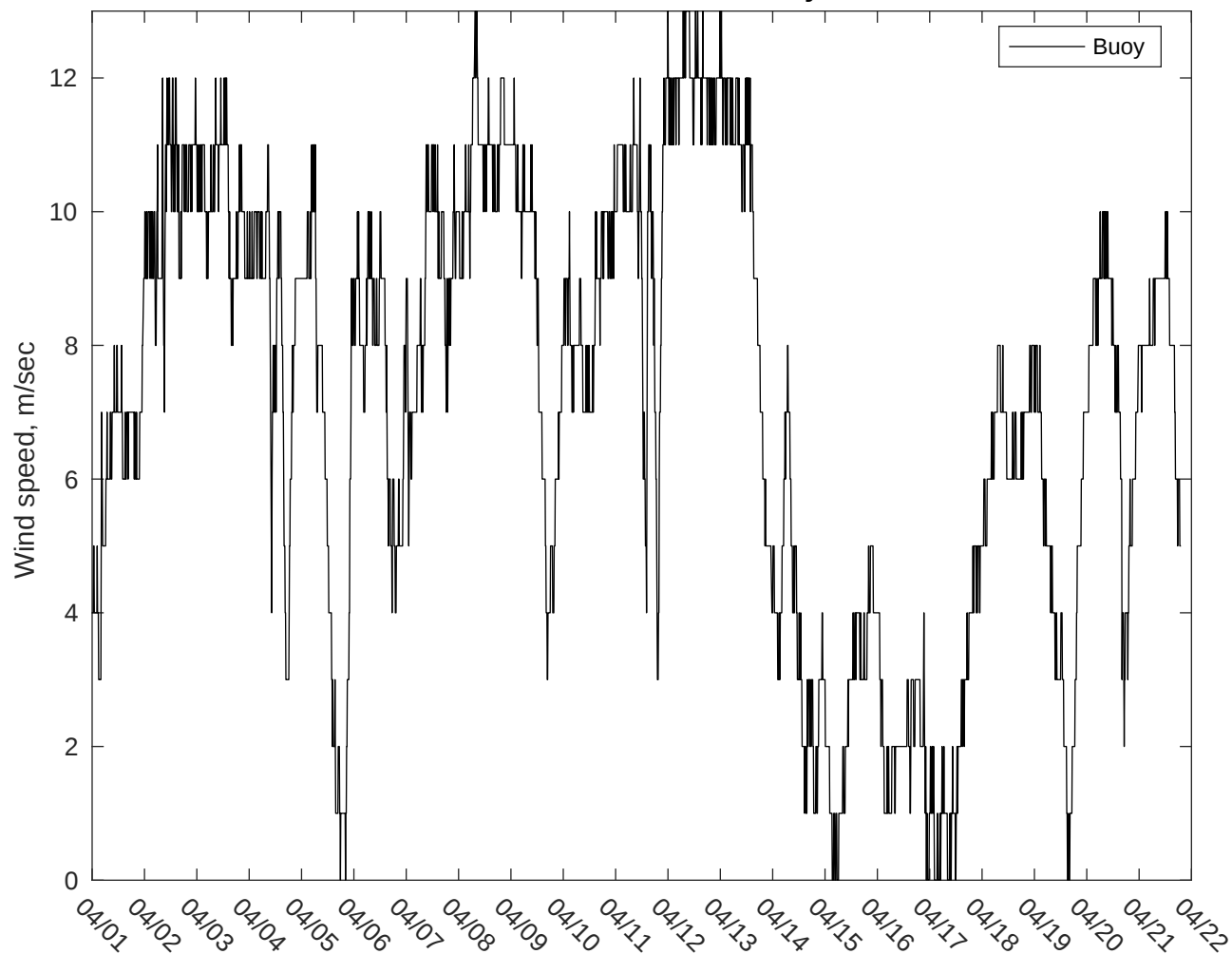
NDBC 46054 vs AUSWAV Winds: 10 to 16 day forecast
