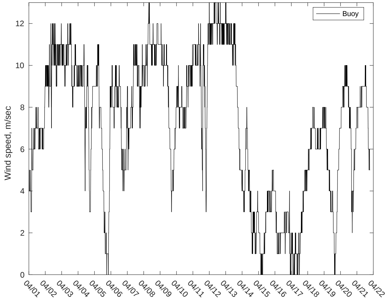
NDBC 46054 vs AUSWAV Winds: 7 to 10 day forecast
