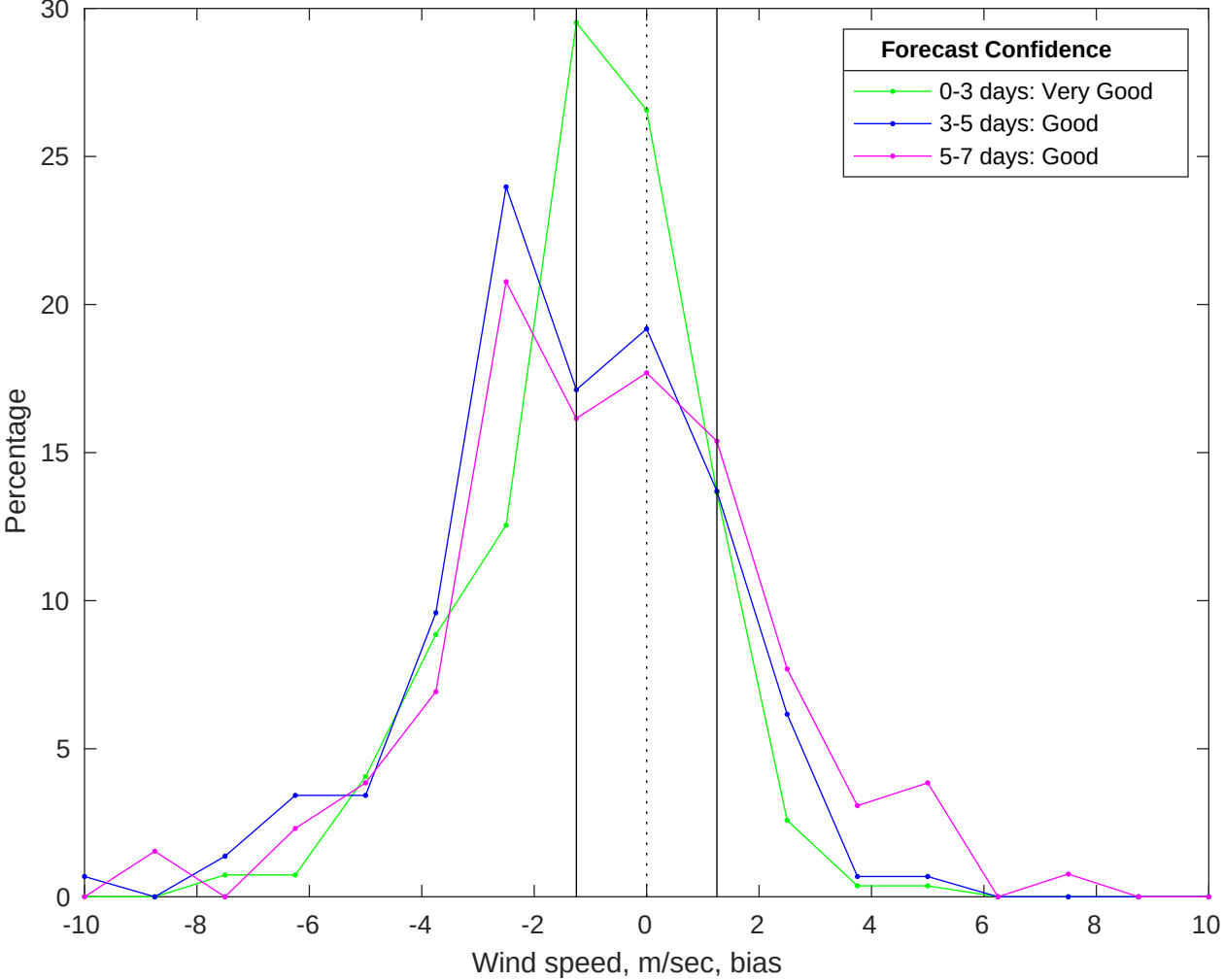
NDBC 46054 vs AUSWAV Winds Bias Histogram: 21-Apr-2025
