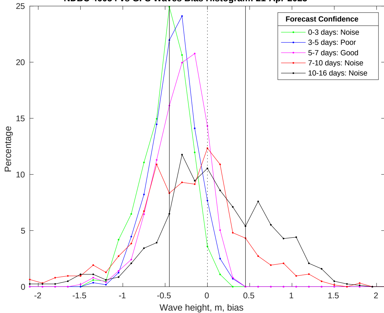
NDBC 46054 vs GFS Waves Bias Histogram: 21-Apr-2025
