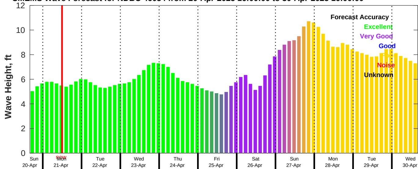
CMEMS Wave Forecast for NDBC 46054 from 20-Apr-2025 16:00:00 to 30-Apr-2025 16:00:00
