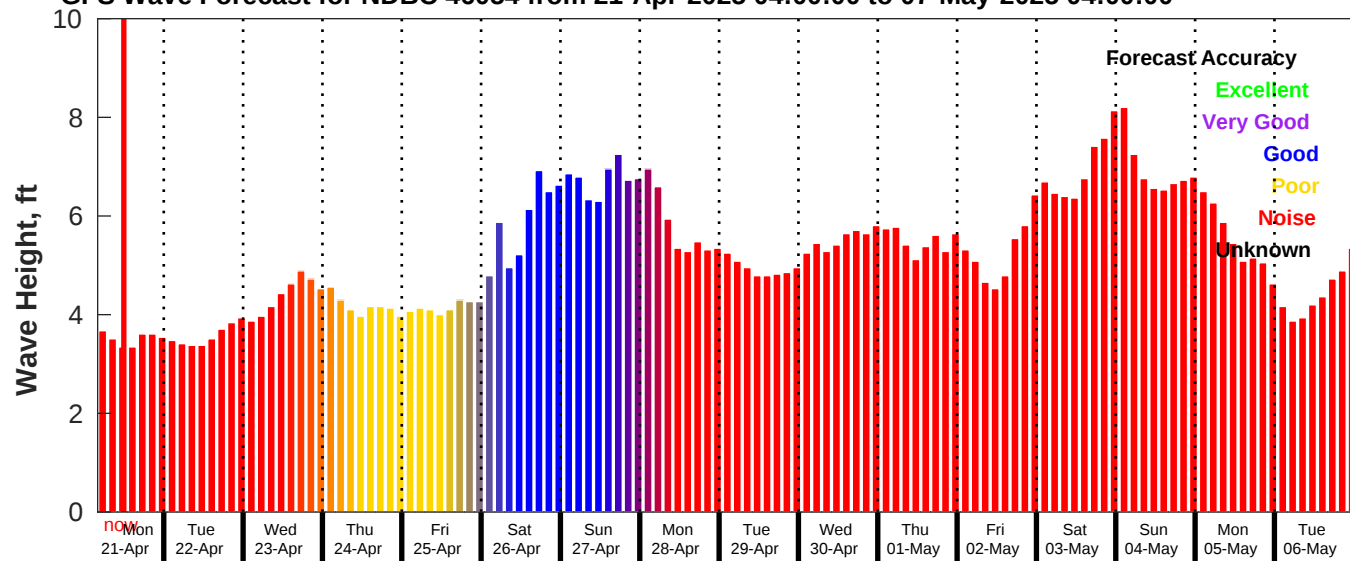
GFS Wave Forecast for NDBC 46054 from 21-Apr-2025 04:00:00 to 07-May-2025 04:00:00
