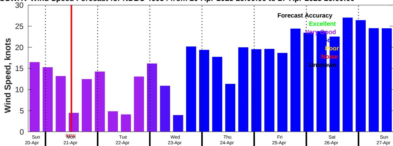
AUSWAV Wind Speed Forecast for NDBC 46054 from 20-Apr-2025 16:00:00 to 27-Apr-2025 16:00:00
