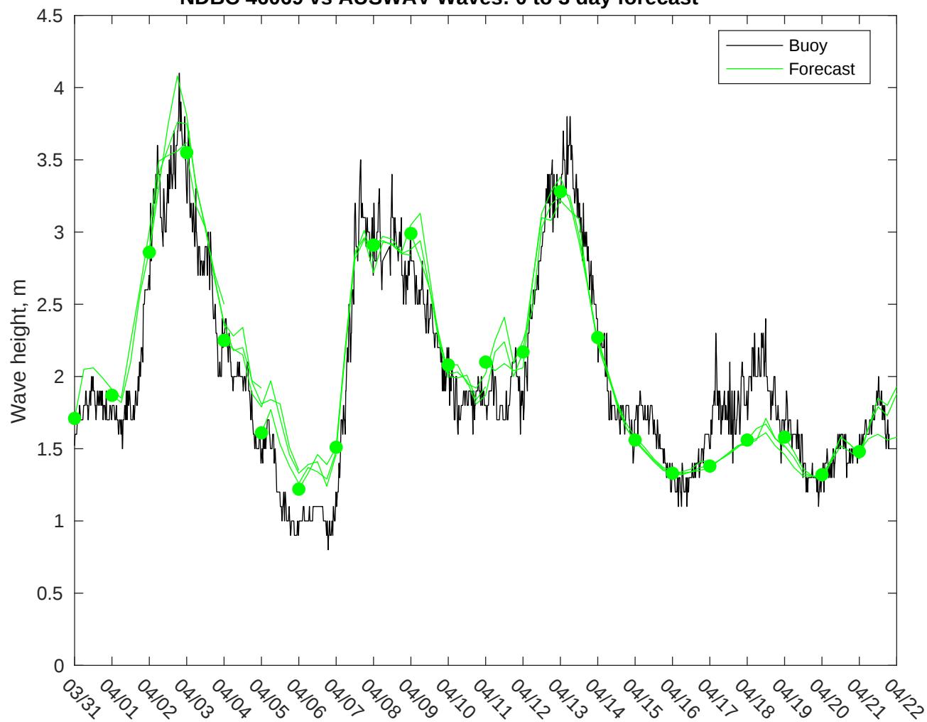
NDBC 46069 vs AUSWAV Waves: 0 to 3 day forecast
